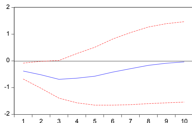
Accumulated Response of SUICIDIOMASC to POVERTYGAP
