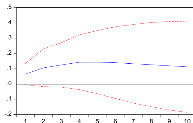
Accumulated Response of SUICIDIOFEME to POVERTYGAP
